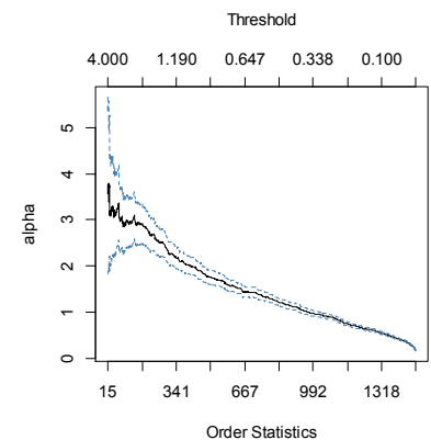
Figure 4. The variation of the Hill estimator
