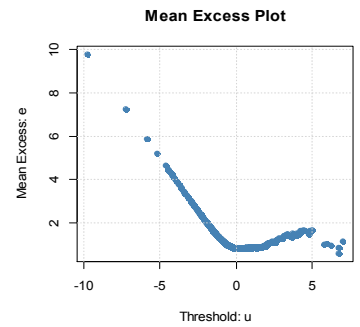
Figure 3. The MEF plots
