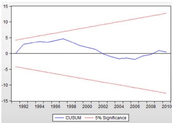
Figure 1. CUSUM Test for stability of parameters.
